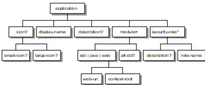
Figure 23. J2EE:1.2 application XML DTD Structure
