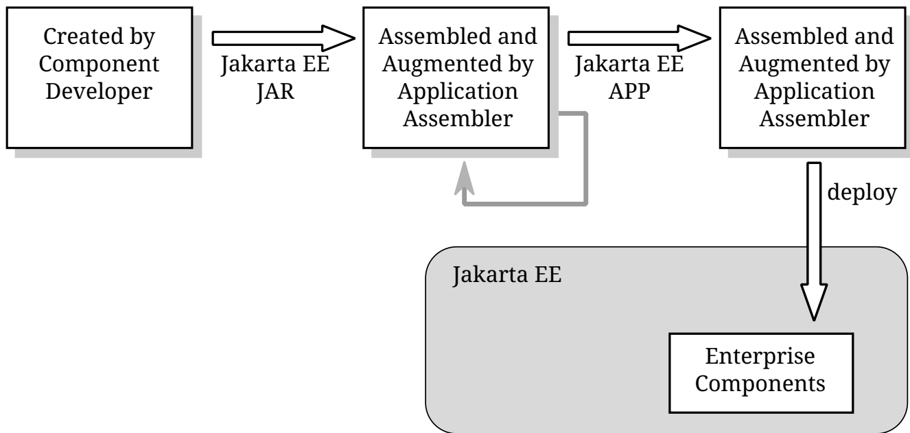
Figure 10. Jakarta EE Application Life Cycle
