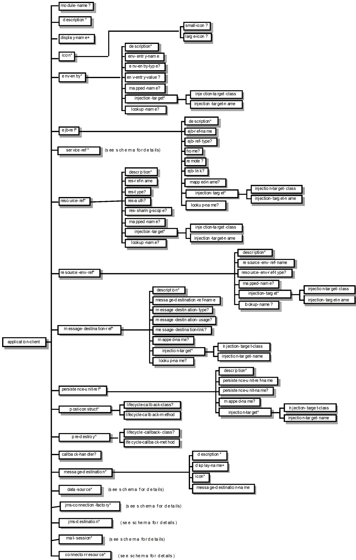
Figure 12. Jakarta EE Application Client XML Schema Structure
