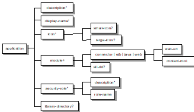
Figure 17. Java EE 5 Application XML Schema Structure
