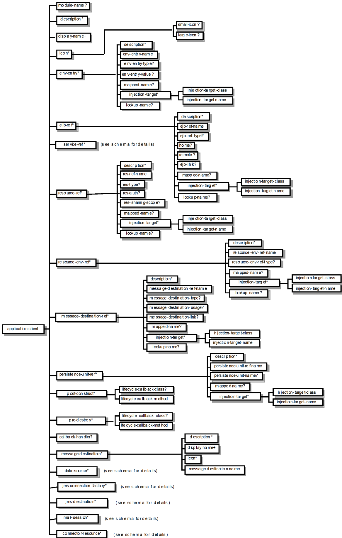
Figure 14. Java EE 7 Application Client XML Schema Structure
