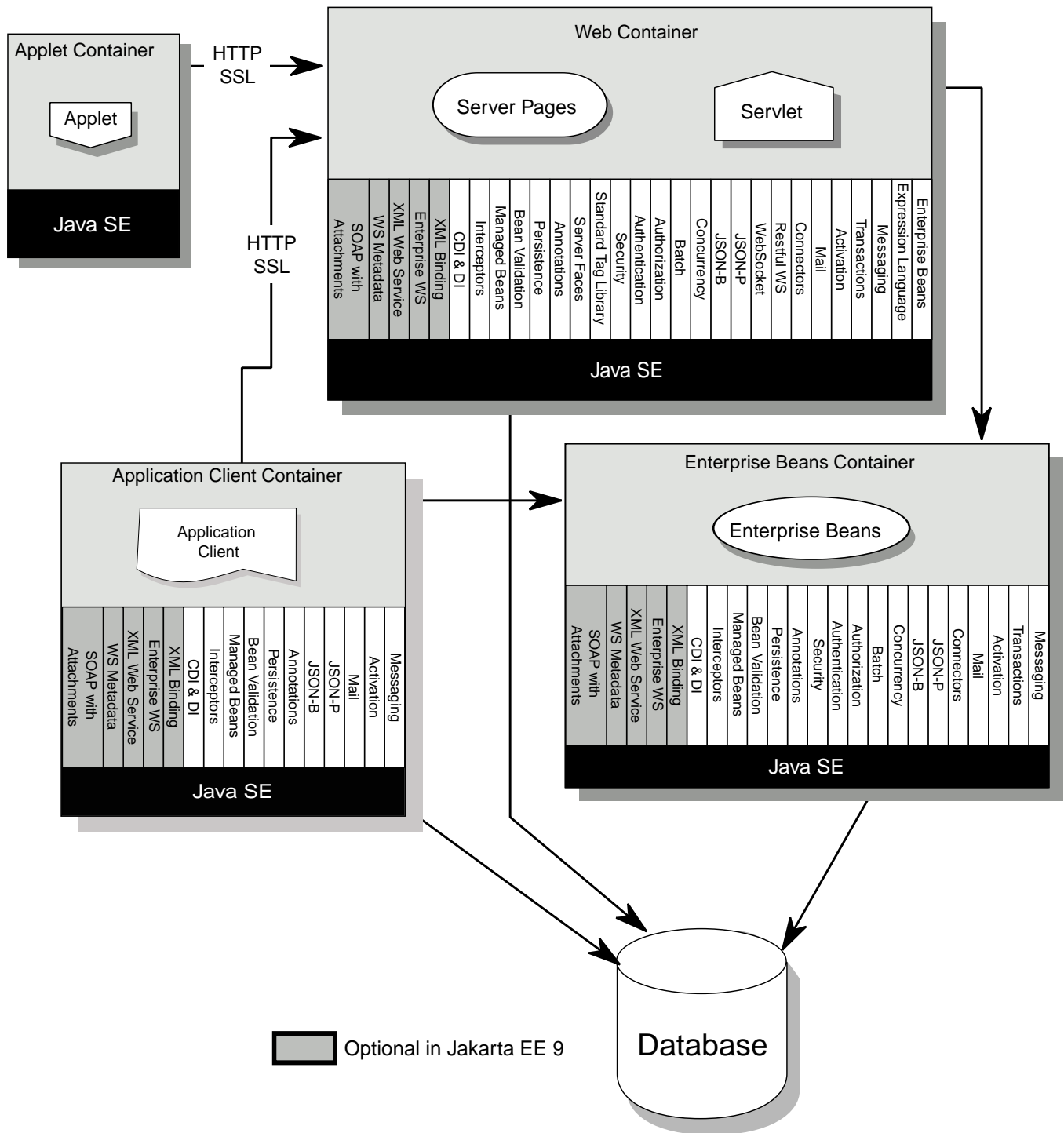
Figure 1. Jakarta EE Architecture Diagram
