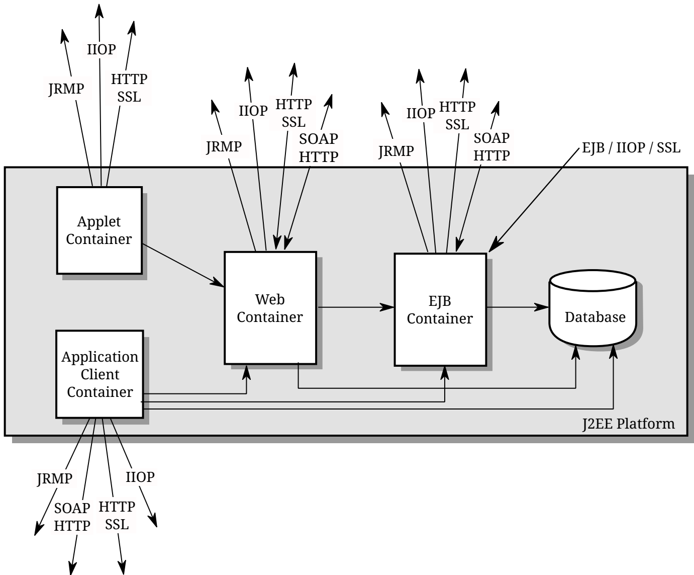
Figure 2. Jakarta EE Interoperability
