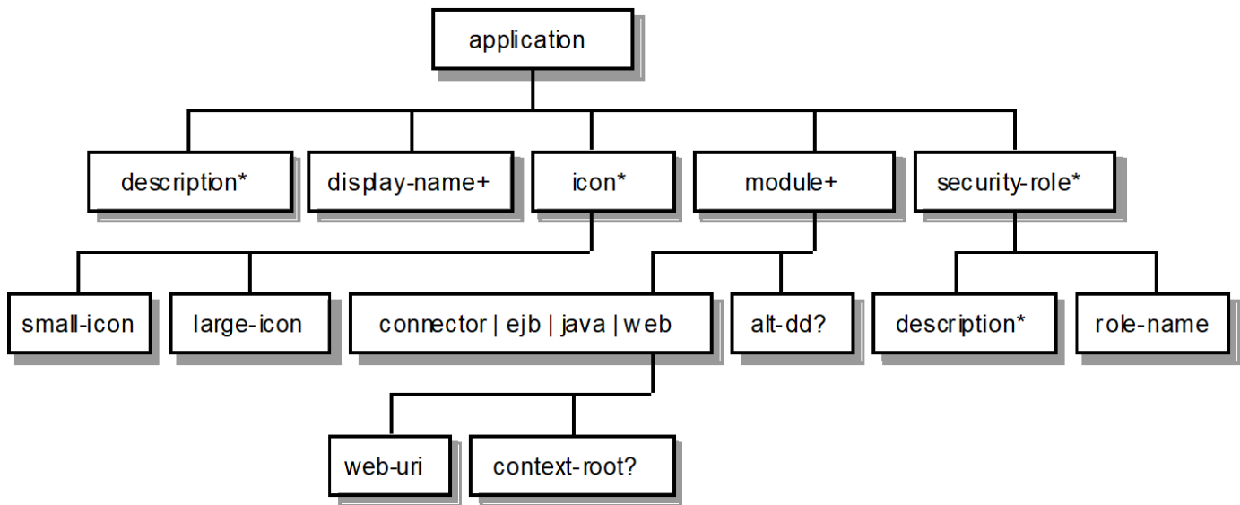
Figure 21. J2EE:1.3 application XML DTD Structure
