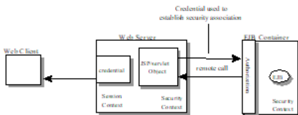
Figure 7. Invoking an Enterprise Bean Business Method
