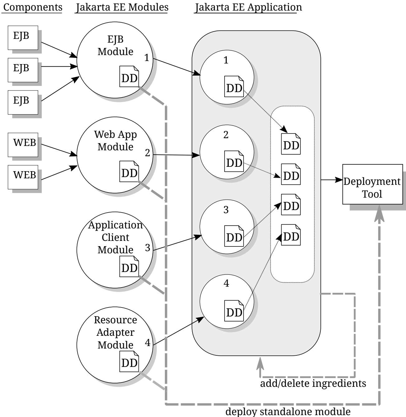
Figure 9. Jakarta EE Deployment
