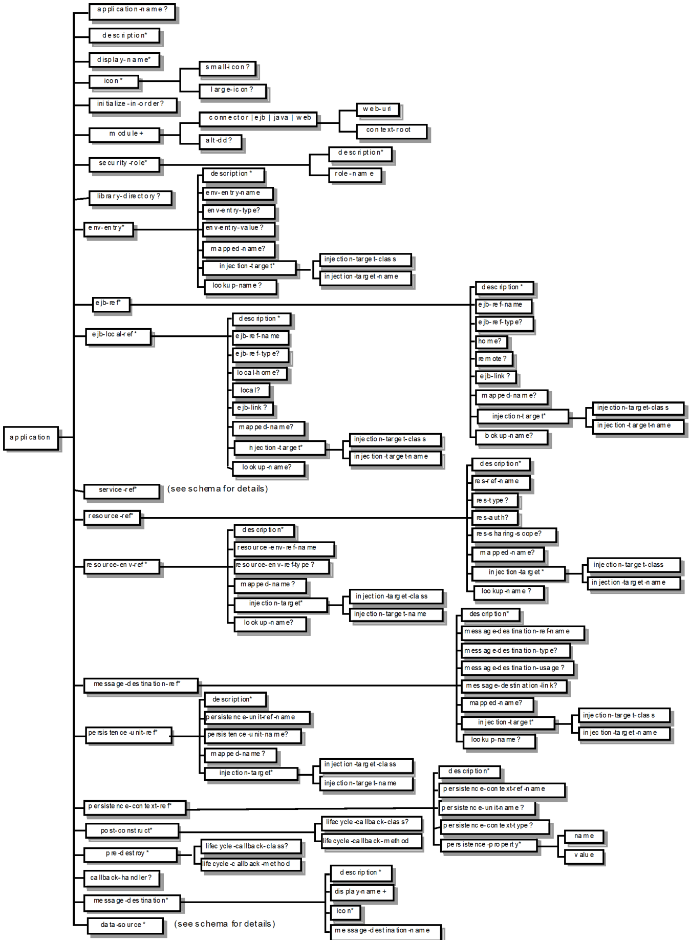
Figure 15. Java EE 6 Application XML Schema Structure
