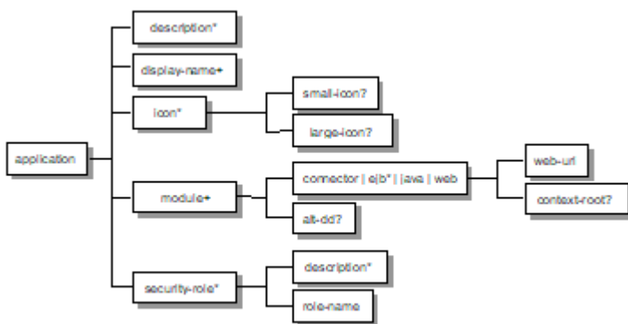
Figure 19. J2EE 1.4 Application XML Schema Structure
