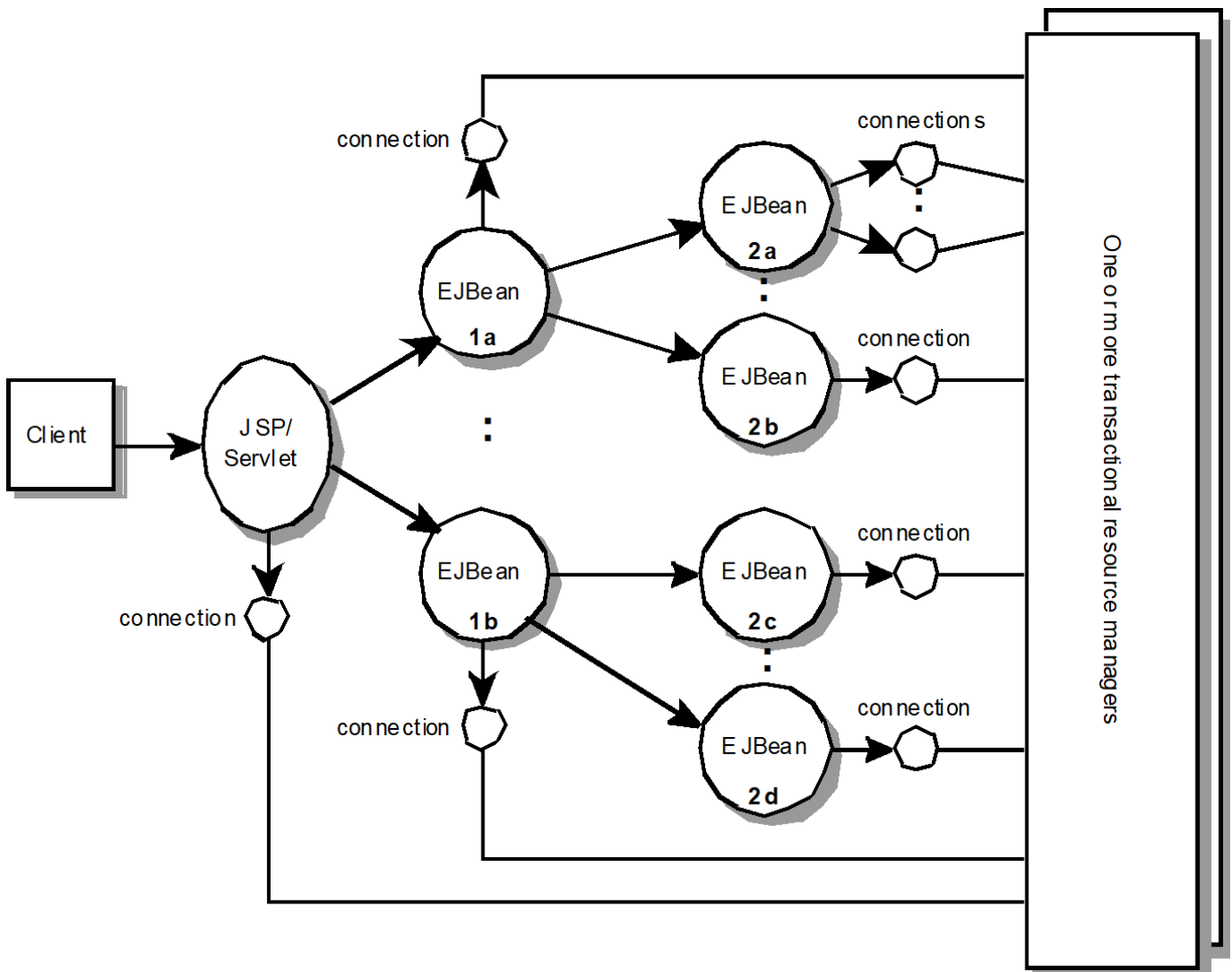
Figure 8. Servlets/Server Pages Accessing Enterprise Beans
