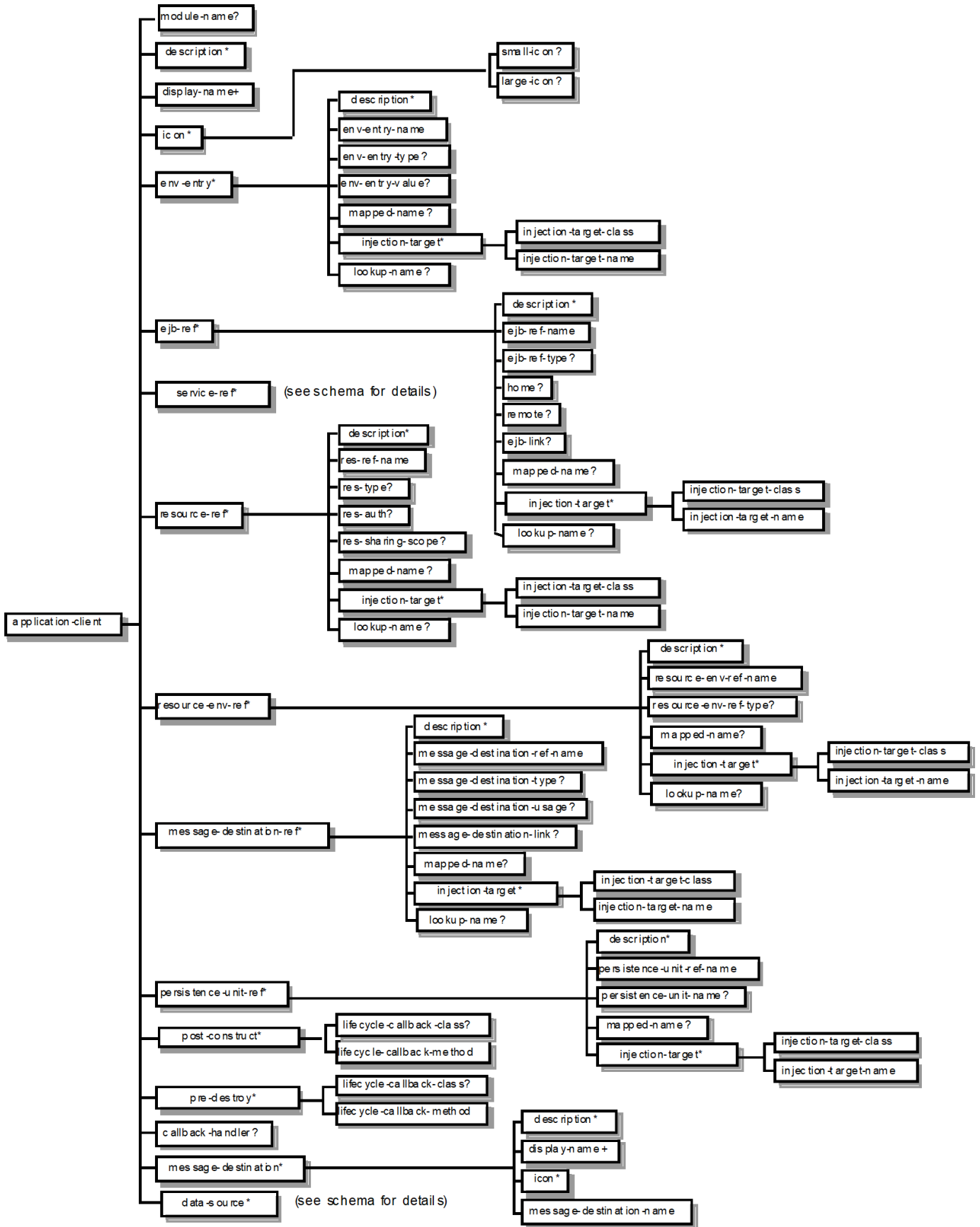
Figure 16. Java EE 6 Application Client XML Schema Structure
