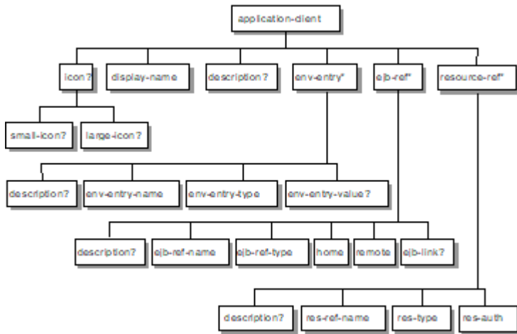
Figure 24. J2EE:1.2 application-client XML DTD Structure
