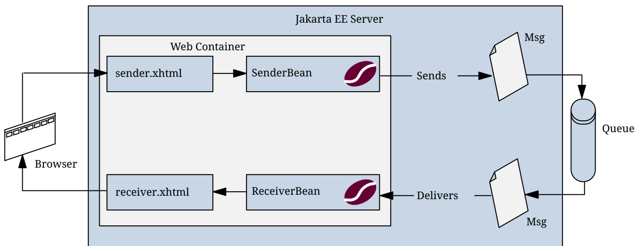
Figure 33. The websimplemessage Application
